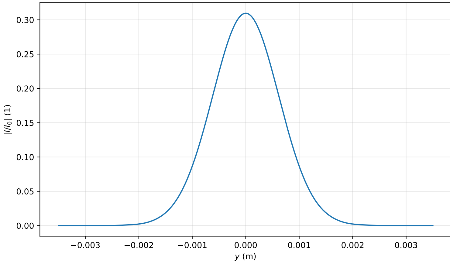
Intensity profile I(x=0, y, z=3.184)/I_0 , P_{in}=0.1P_{cr} , artificial time
